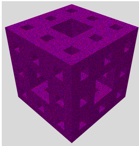
Figure 30.2 A Menger Sponge with the demo meshuppper applied.
